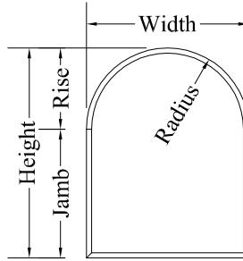
Round Top Picture Window (Rise = 1/2 Width)
