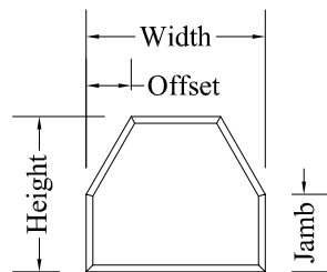
Hex Head
