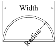
Half Round (Height = 1/2 Width)
