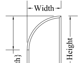
Quarter Round Picture Window
