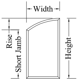
Quarter Segment Top Picture Window
